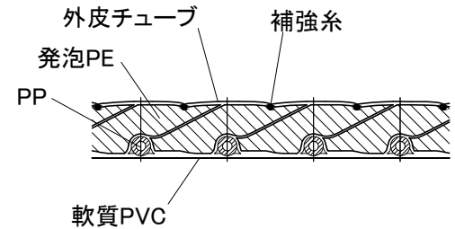
K部詳細 2/1
