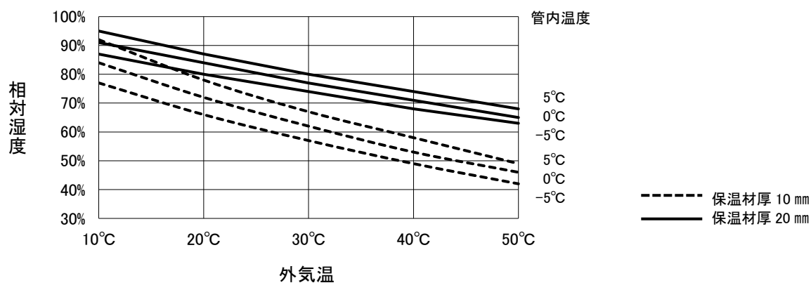
図-10 銅管 \phi 38.10
