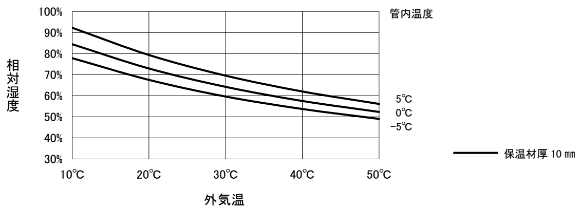
図-6 銅管 \phi 9.52
